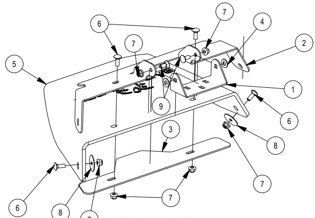
210-6015-98 Discharge Assembly
