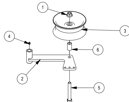
039-6952-23 SD DECK IDLER ASSEMBLY
