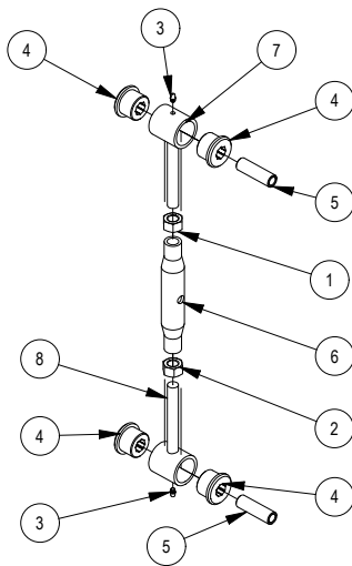
048-7000-00 Turnbuckle
