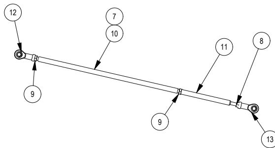
PUSH ROD ASSEMBLY 035-0006-19
