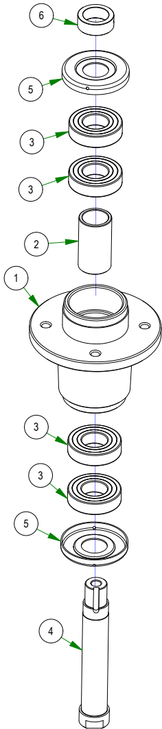
037-4000-00 OUTLAW SPINDLE ASSEMBLY
