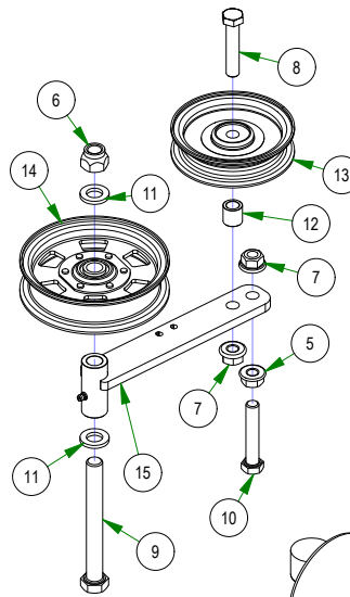
039-5944-05 Maverick Pump Idler
