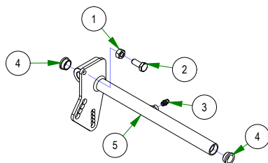
031-0053-21 2021 Maverick Drive Arm Actuator RH Assembly
