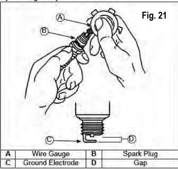
Spark Plug Component and Details
