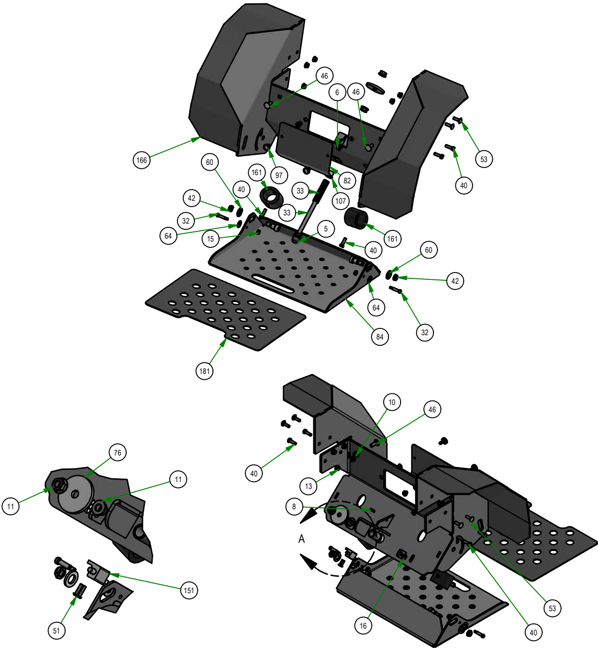
DETAIL A
