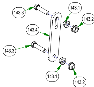
039-2127-17 Deck Hanger Assembly
