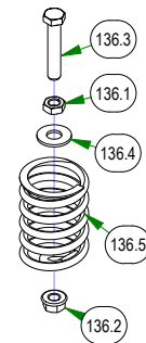
034-8045-03 Seat Spring Assembly
