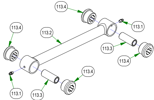
028-0004-22 Hybrid Turnbuckle/Deck Locator
