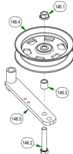
039-6945-18 2017 54"/48" Deck Idler Assembly
