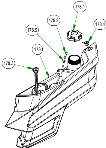
067-2021-00 2021 Maverick Left Side Tank
