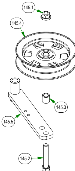
039-6945-17 2017 MZ/ZT Deck Idler Assembly
