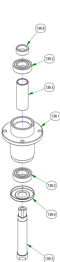
037-6015-50 Spindle Assembly
