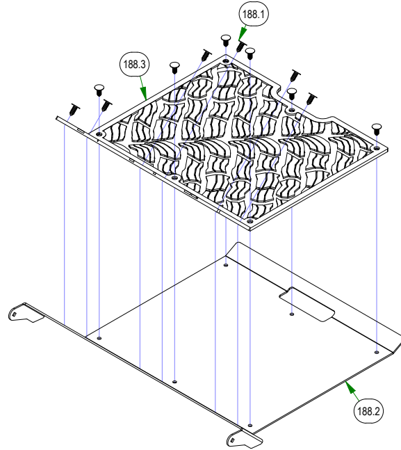
079-3470-21 2021 Maverick Floorboard Assembly
