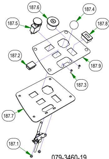
079-3460-19 2019 ZT/Maverick Control Panel Assembly
