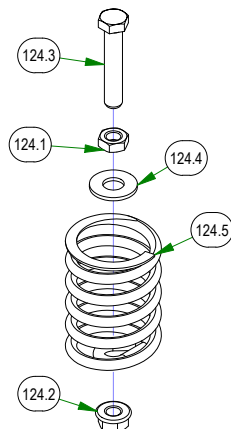
034-8045-03 Seat Spring Assembly
