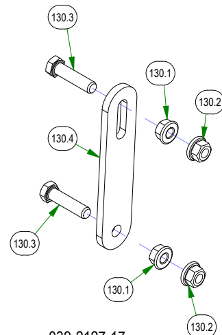
039-2127-17 Deck Hanger Assembly
