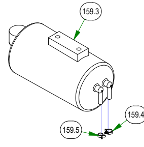
067-0020-01 ZT/Mav EPA Cannister Assy
