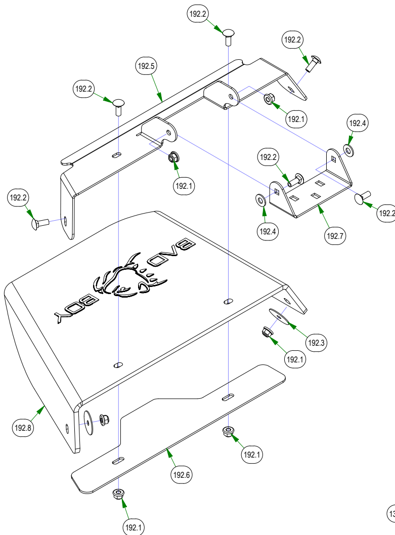
210-6015-98 MZ Discharge Chute Assembly
