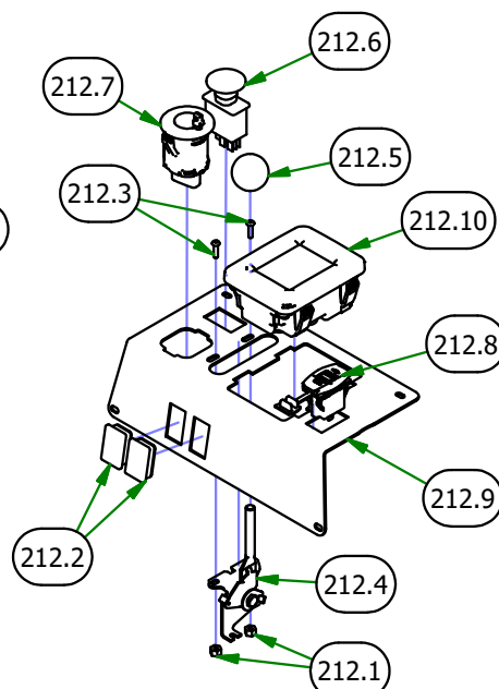
079-3482-19 Renegade Control Panel Assembly
