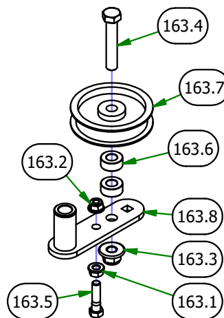
039-6950-99 2019 Renegade Belt Tensioner LH
