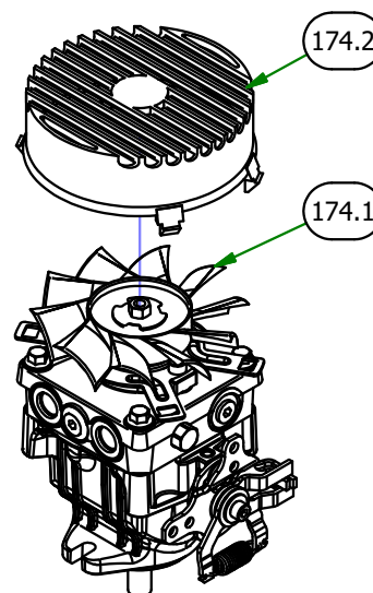
050-3003-00 2019 Outlaw Renegade Right Pump 16cc
