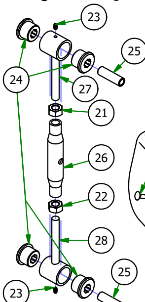
048-7000-00 Turnbuckle
