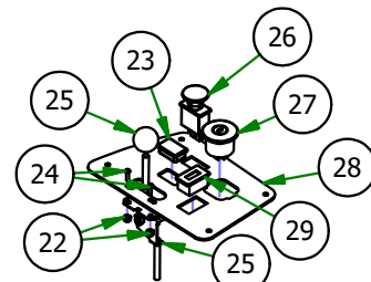
079-3460-01 2017 Magnum Control Panel Assembly
