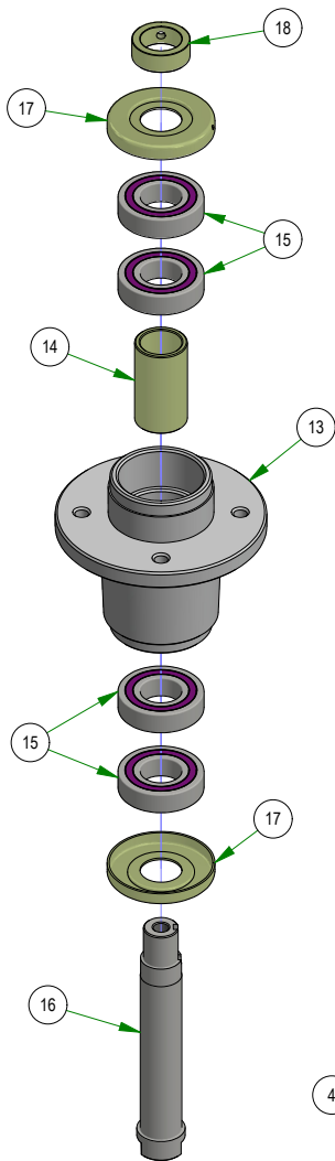
037-4000-00 SPINDLE ASSEMBLY
