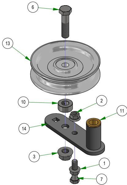
039-6950-94 RIGHT PUMP IDLER
