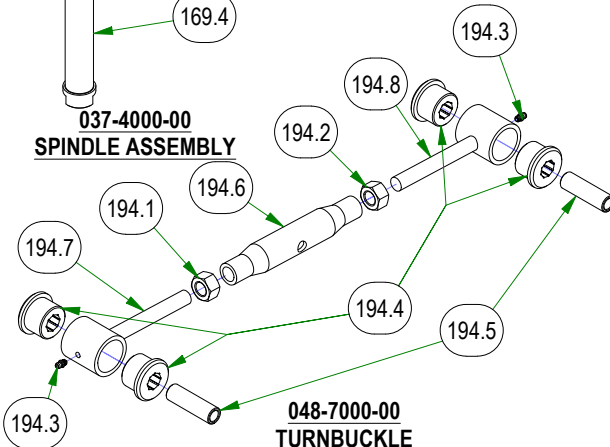
039-2125-17 DECK HANGER
