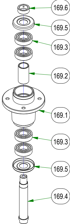
037-4000-00 SPINDLE ASSEMBLY
