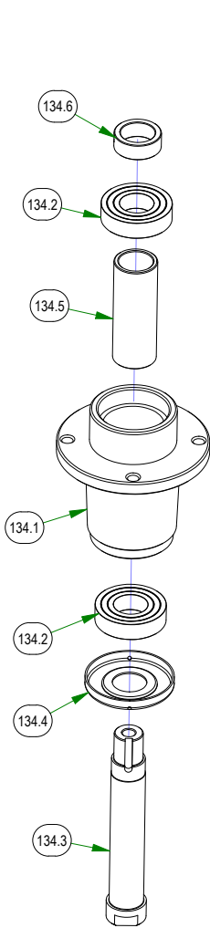
037-6015-50 Spindle Assembly
