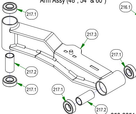
250-2851-21 2021 Maverick RH Long Front Suspension Arm Assy (54" & 60")
